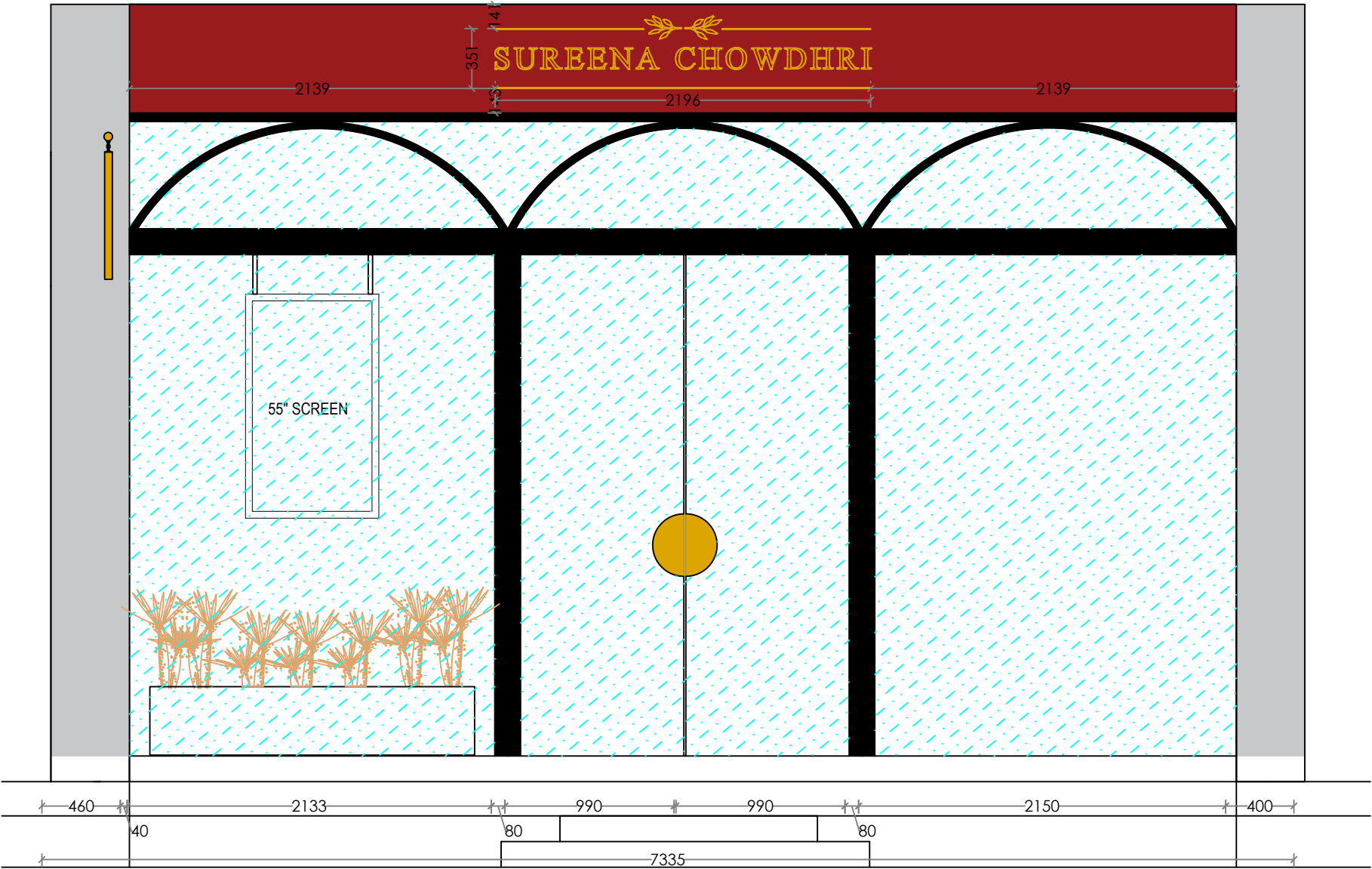
EXTERNAL FACADE ELEVATION WITH PROPOSED SIGNAGE
