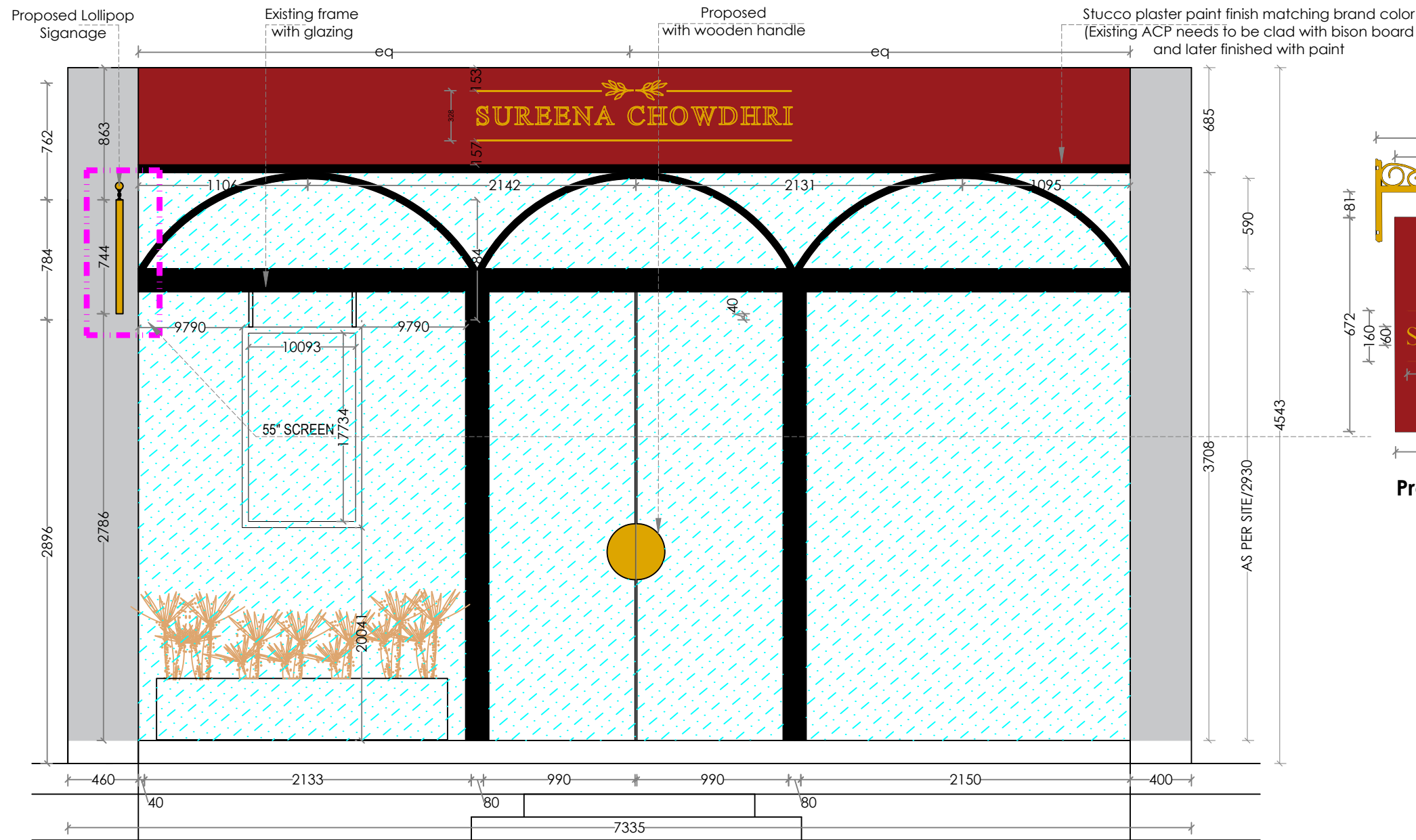
EXTERNAL FACADE ELEVATION
