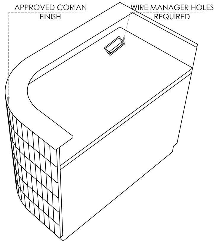
ISO - REAR VEIW
