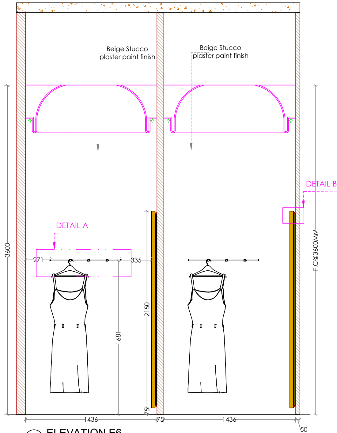
6 ELEVATION E6 Scale: NTS
