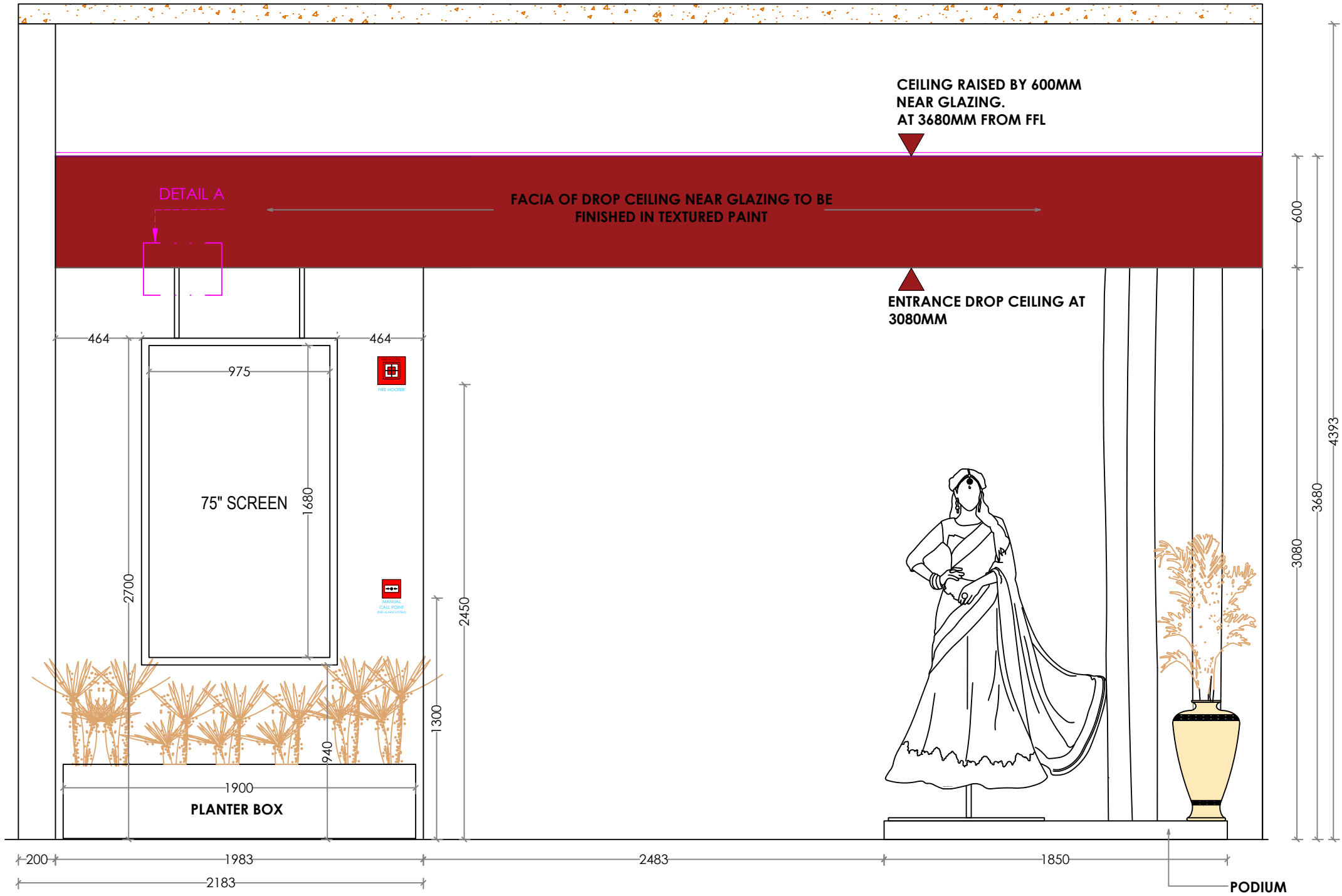
10 ELEVATION S10 Scale: NTS
