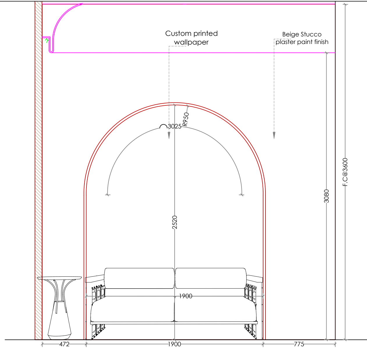
9 ELEVATION E9 Scale: NTS
